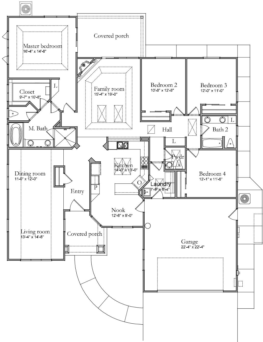
PLAN 7 – ELEVATION A - 4BR/2.5 BA - 2410 SF
